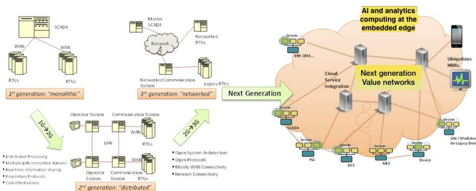
Figure 5 – Evolution of the control systems from different computing architecture generations (monolithic, distributed, networked) to an edge computing one where data analysis, based on AI, is performed close to the end-devices and/or subsystems.
